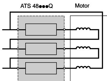
Figure 1 Special use: starter connected to the motor delta terminal in series with each winding
