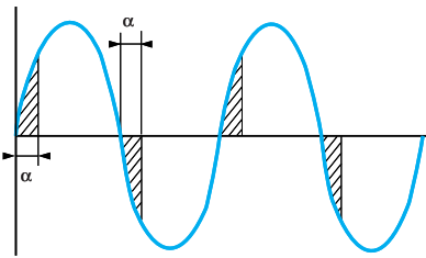
Firing angle
