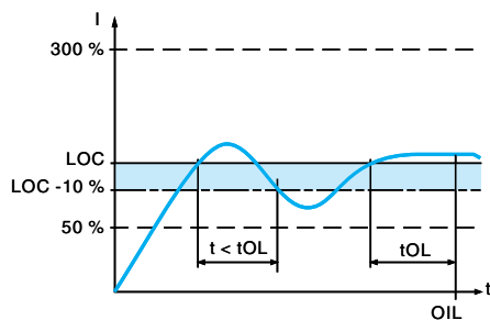
Motor overcurrent detection (OIL)
