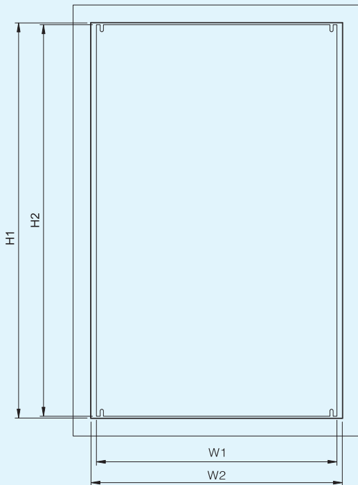
FRONT VIEW (WITHOUT DOOR)
