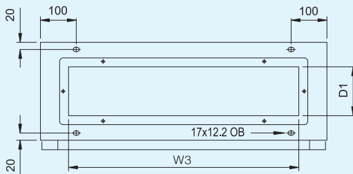
BOTTOM GLAND PLATE & FOUNDATION
