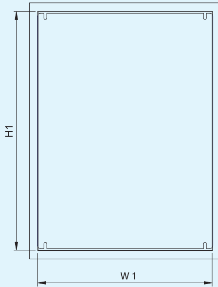
BOTTOM GLAND PLATE
